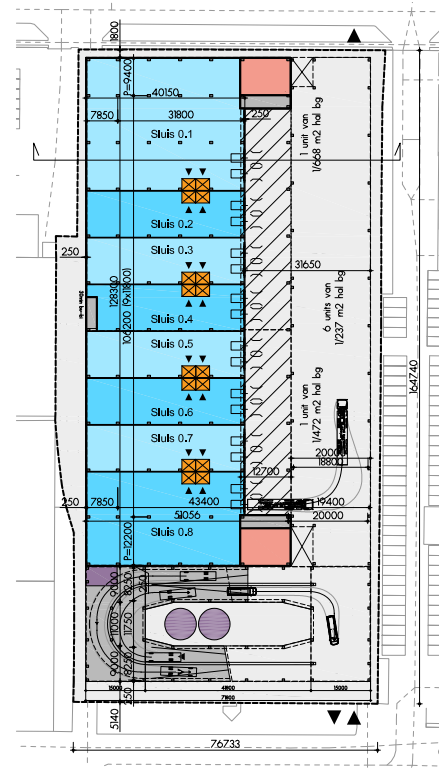
hal
