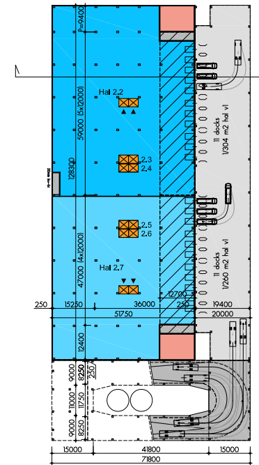
hal/laaddek
