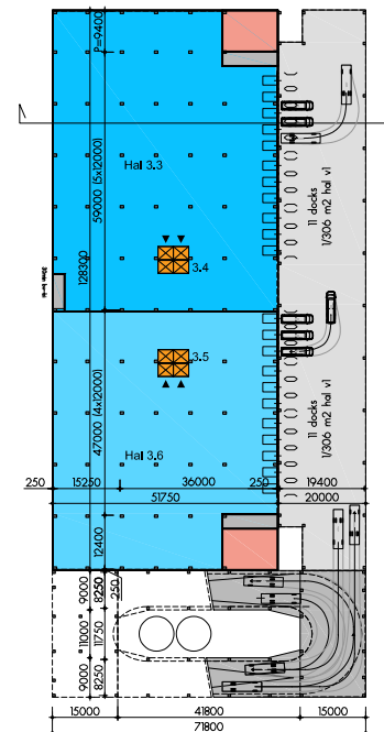
hal/laaddek
